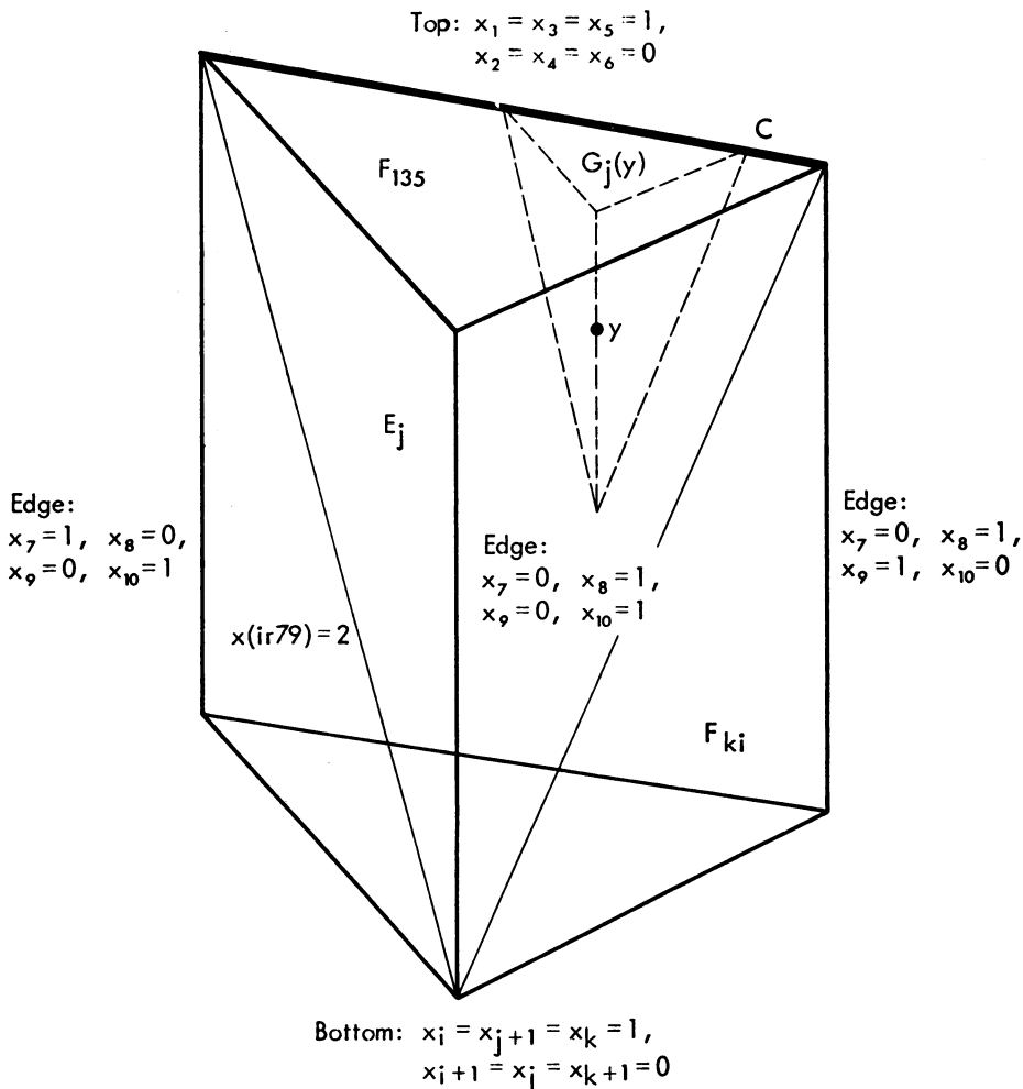
FIGURE 2. Regions E_j , F_{135} , and G_j(y) .
